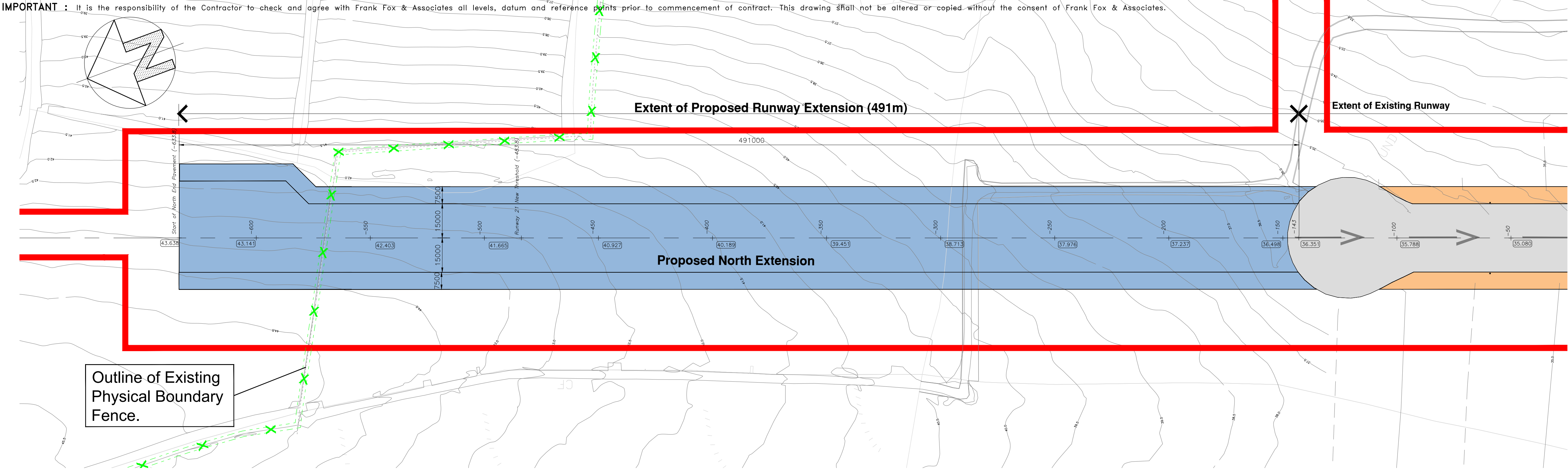
GENERAL ARRANGEMENT NORTH END RUNWAY EXTENSION LAYOUT
